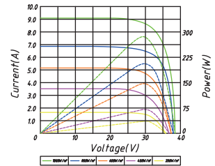
I-V CURVE TP660P Pm(W)260
